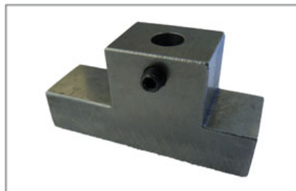
T016-884-20 BOSCH EUI/EUP ARMATURE GAP MEASURING ADAPTOR
