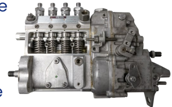
Zexel 4 Cylinder
