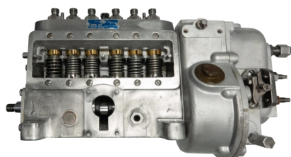
C.A.V 6 Cylinder
